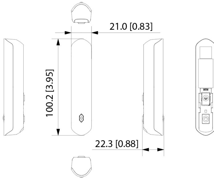
Figure 3-1 Dimensions (Unit: mm[inch])
